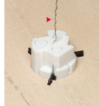
3 Wrap drop wire twice through loop on top of box and around a framing member above ceiling. Wrap wire around itself six times minimum in both instances.
